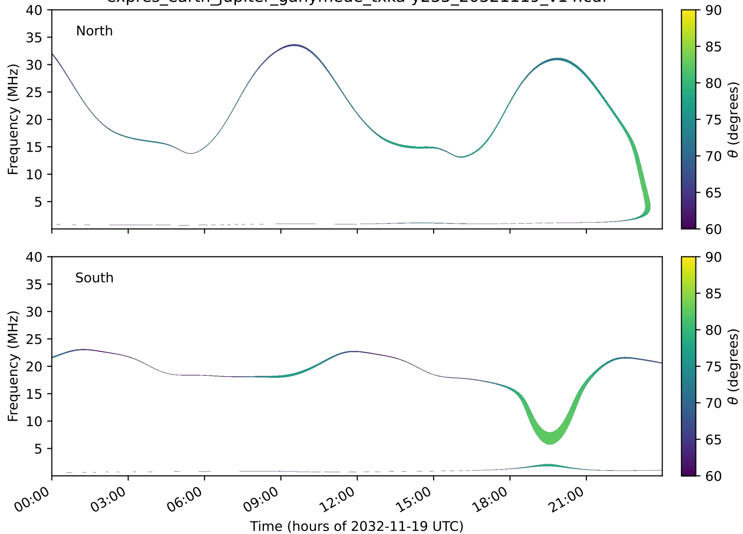
expres_earth_jupiter_ganymede_txka-y235_20321119_v14.cdf
