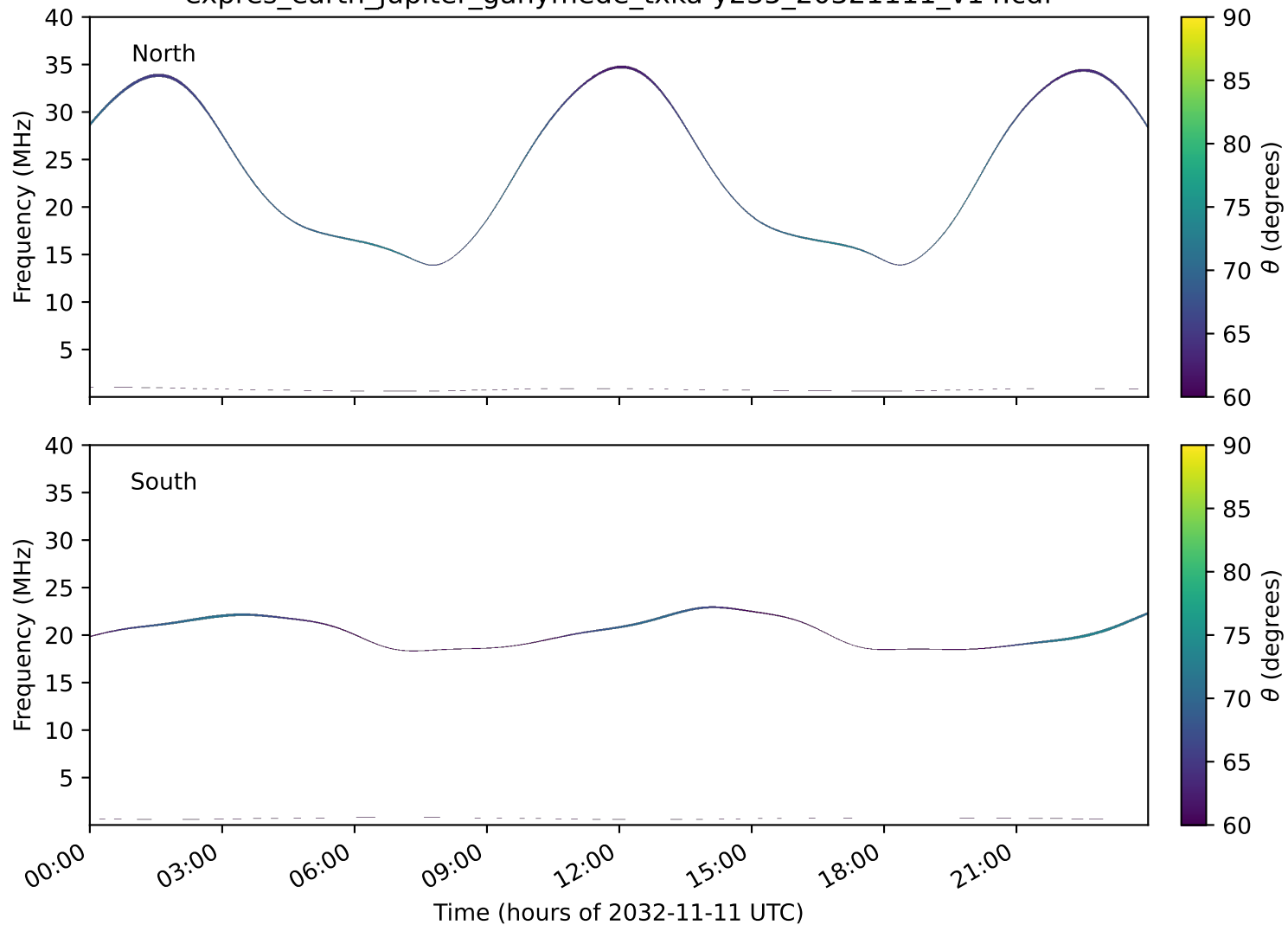
expres_earth_jupiter_ganymede_txka-y235_20321111_v14.cdf
