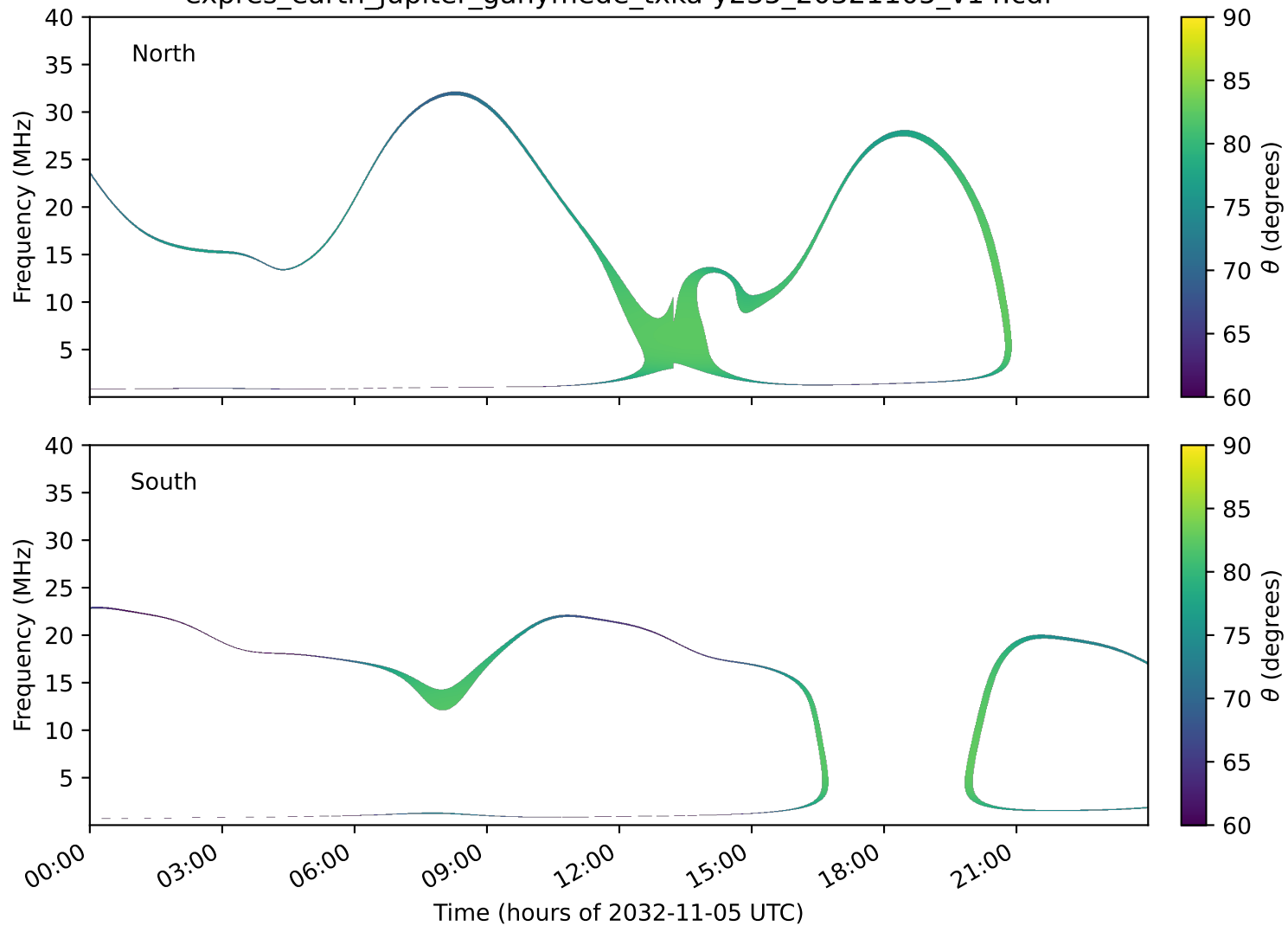
expres_earth_jupiter_ganymede_txka-y235_20321105_v14.cdf
