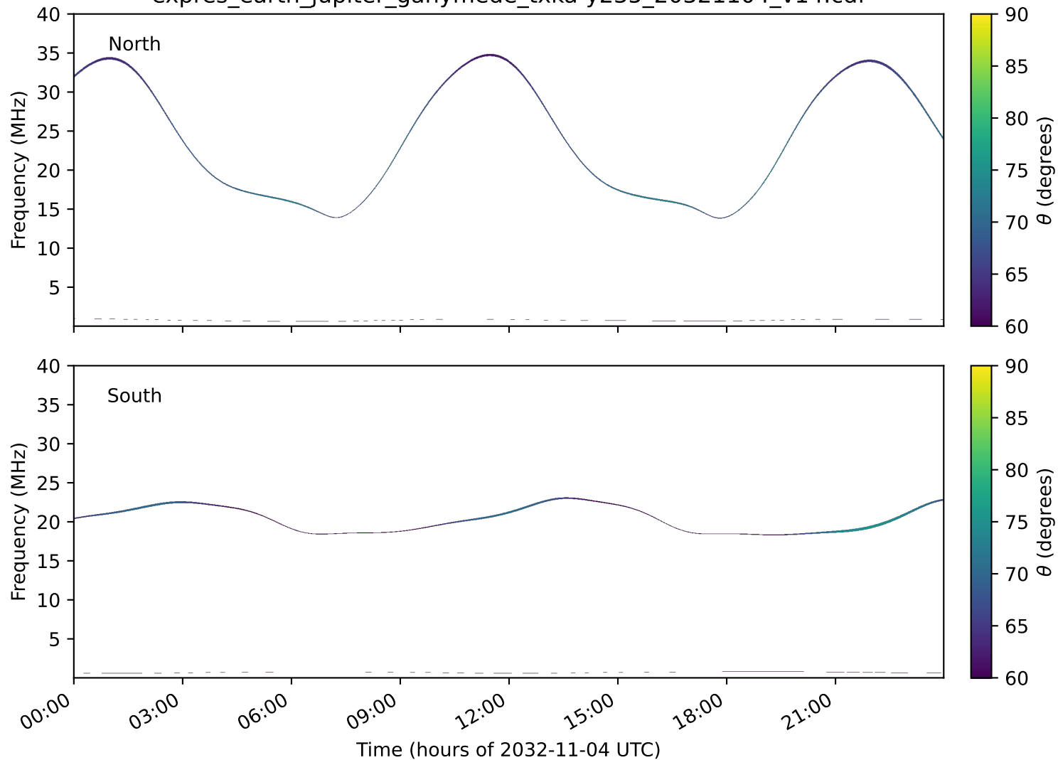
expres_earth_jupiter_ganymede_txka-y235_20321104_v14.cdf
