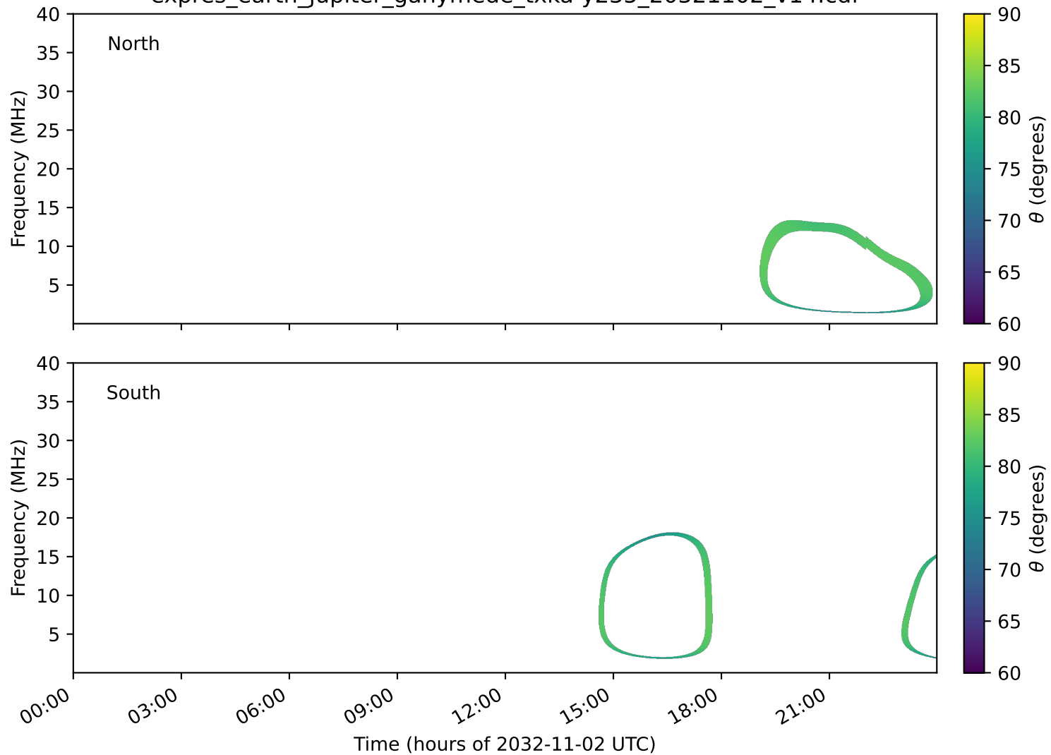
expres_earth_jupiter_ganymede_txka-y235_20321102_v14.cdf
