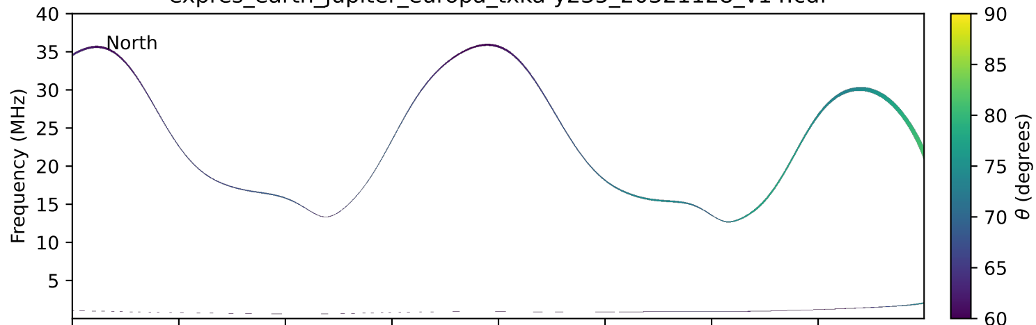
expres_earth_jupiter_europa_txka-y235_20321128_v14.cdf
