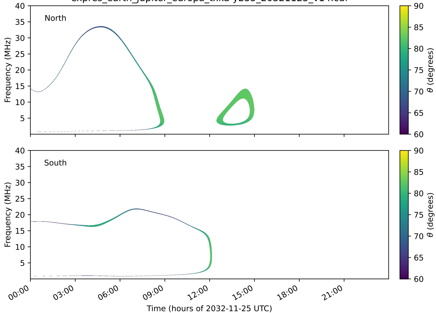
expres_earth_jupiter_europa_txka-y235_20321125_v14.cdf
