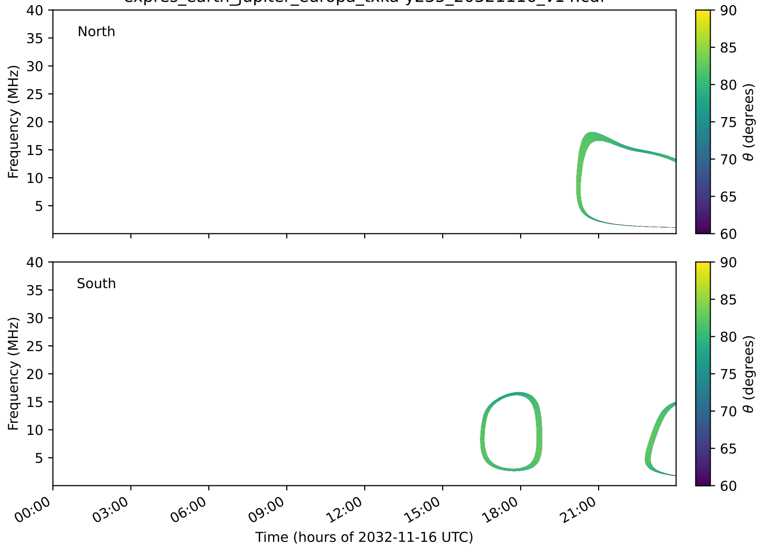
expres_earth_jupiter_europa_txka-y235_20321116_v14.cdf
