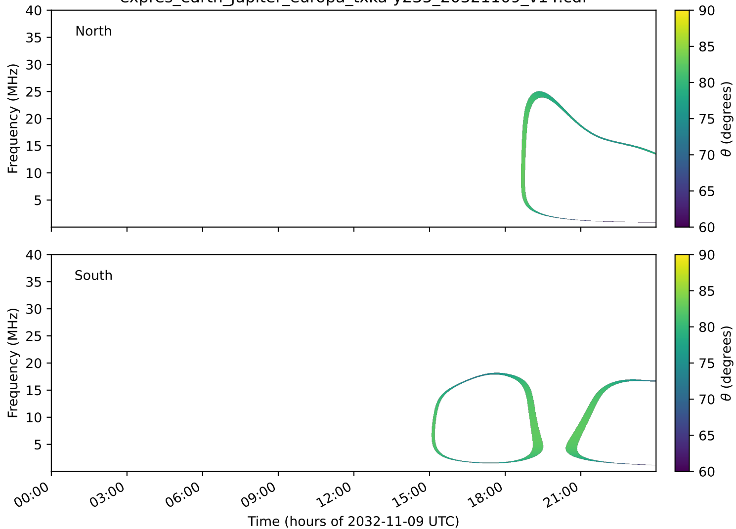
expres_earth_jupiter_europa_txka-y235_20321109_v14.cdf
