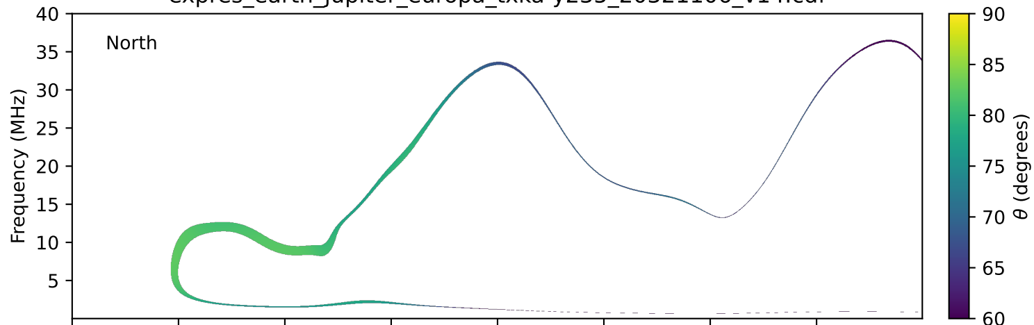
expres_earth_jupiter_europa_txka-y235_20321106_v14.cdf
