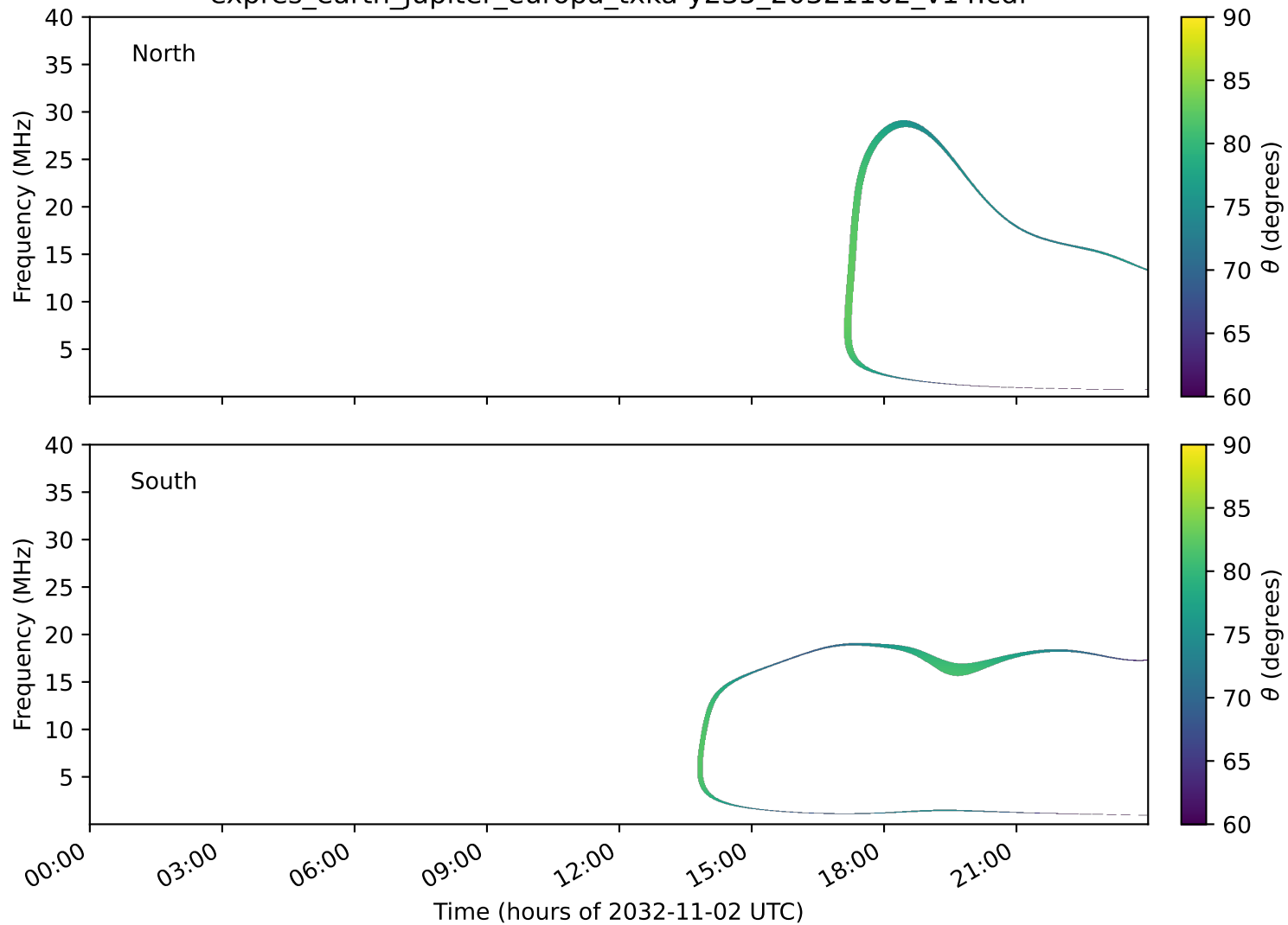
expres_earth_jupiter_europa_txka-y235_20321102_v14.cdf
