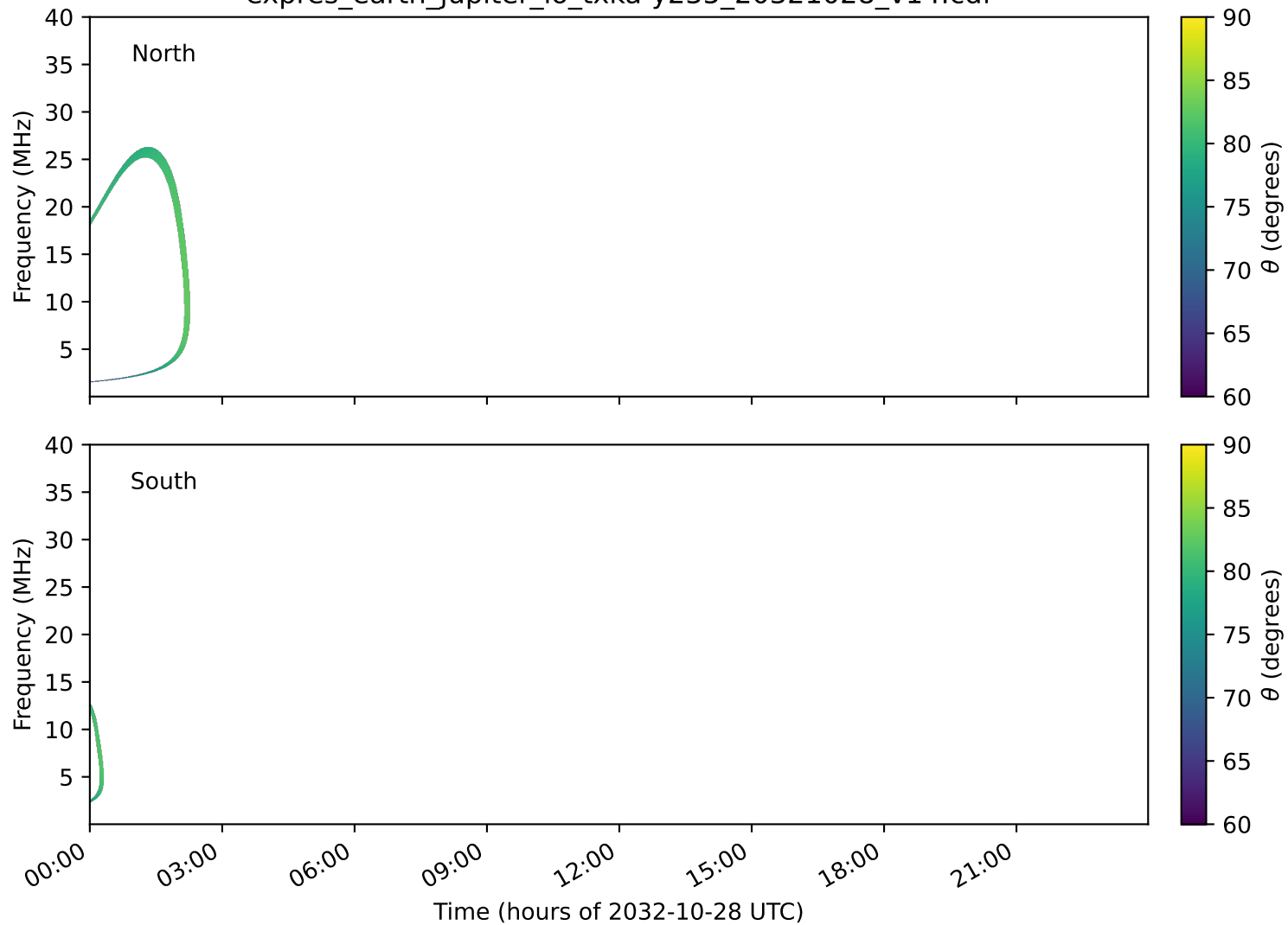
expres_earth_jupiter_io_txka-y235_20321028_v14.cdf
