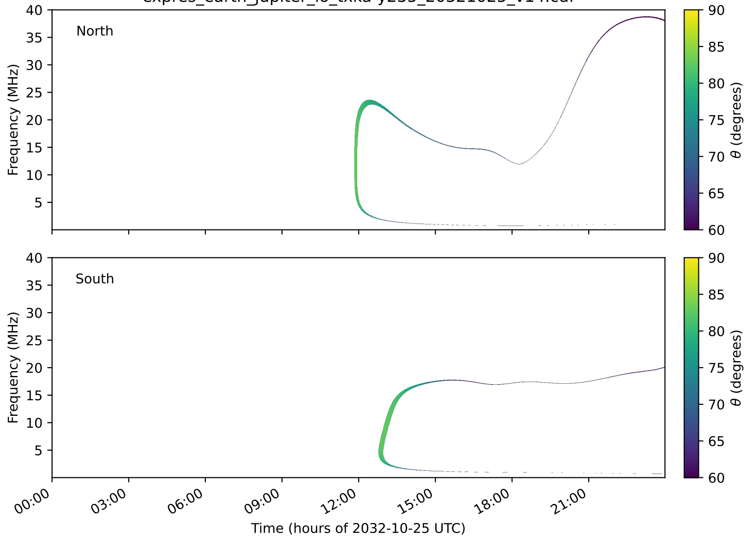
expres_earth_jupiter_io_txka-y235_20321025_v14.cdf
