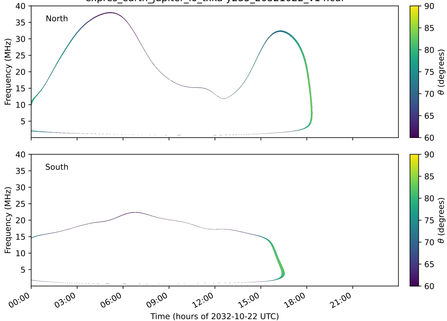
expres_earth_jupiter_io_txka-y235_20321022_v14.cdf
