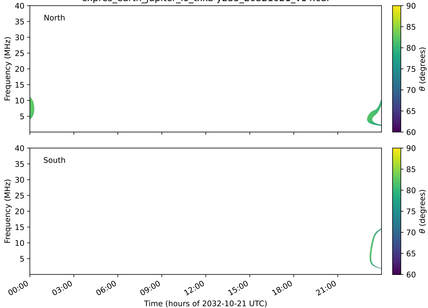
expres_earth_jupiter_io_txka-y235_20321021_v14.cdf
