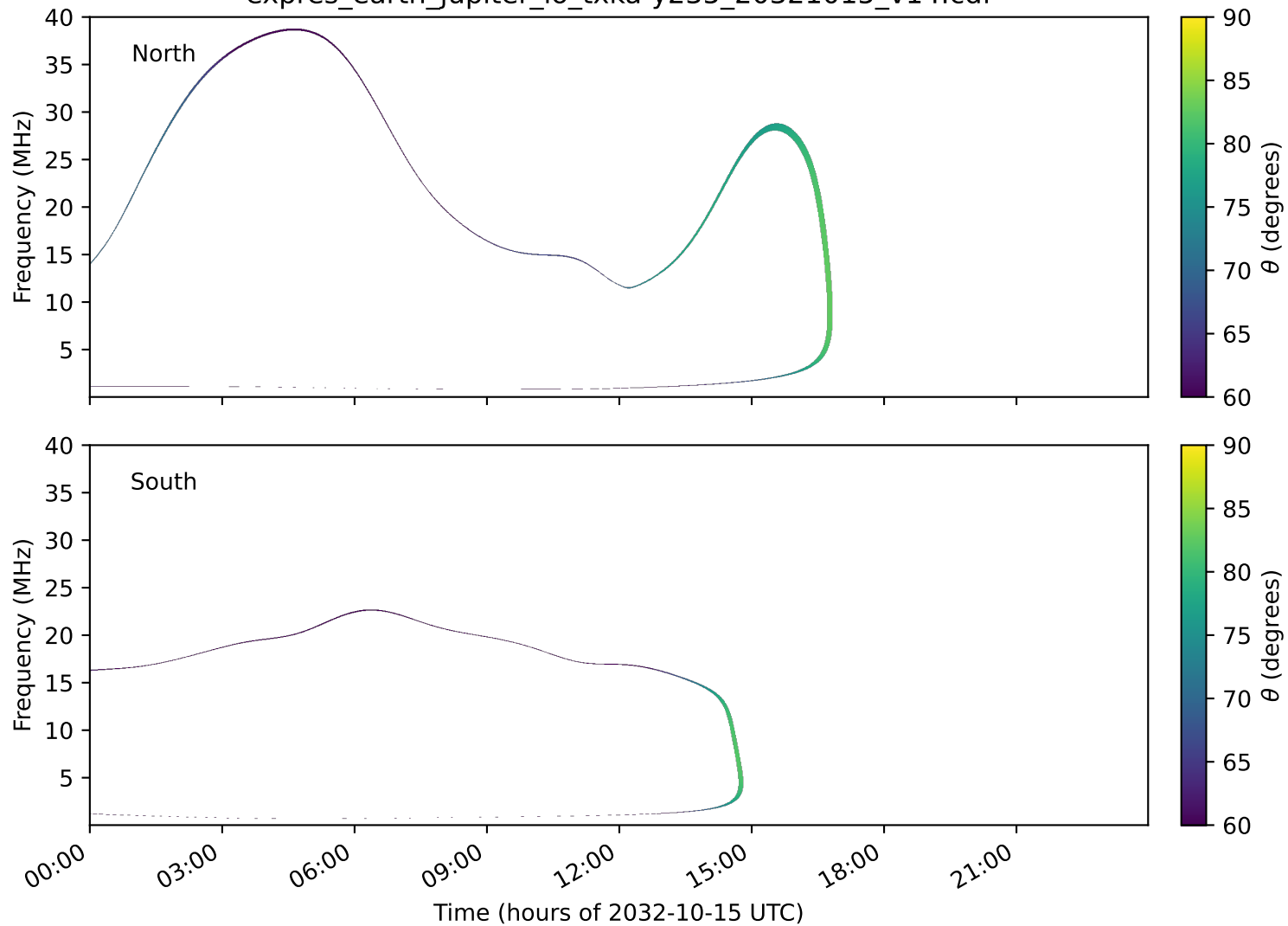
expres_earth_jupiter_io_txka-y235_20321015_v14.cdf
