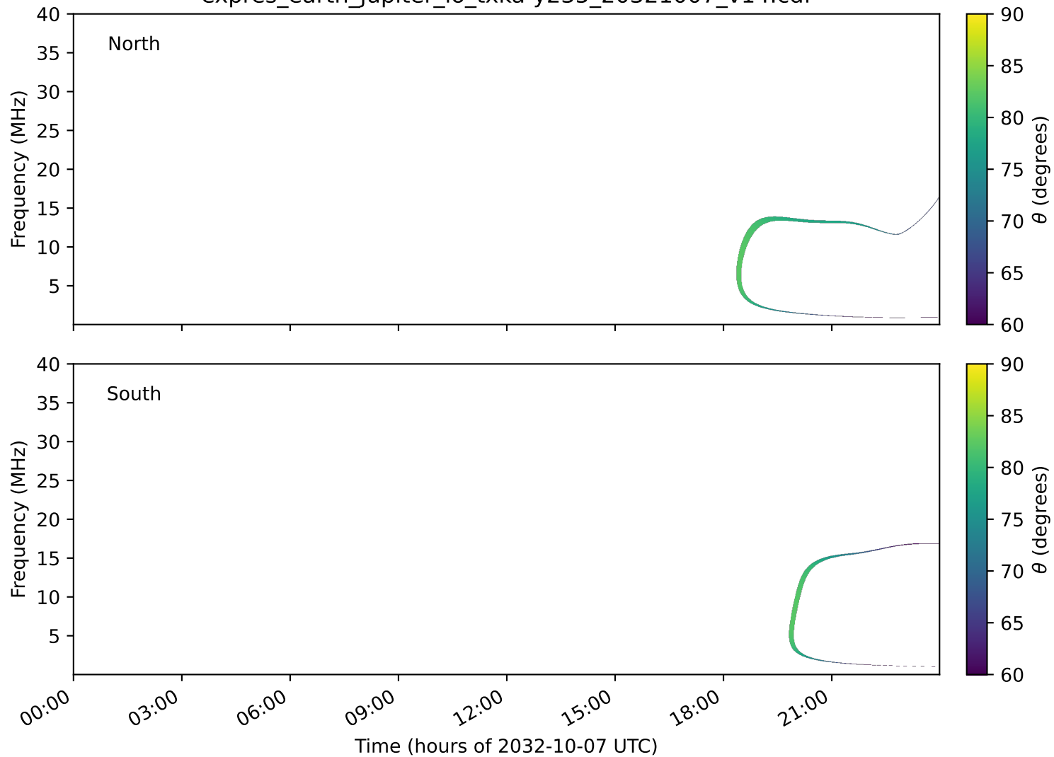
expres_earth_jupiter_io_txka-y235_20321007_v14.cdf
