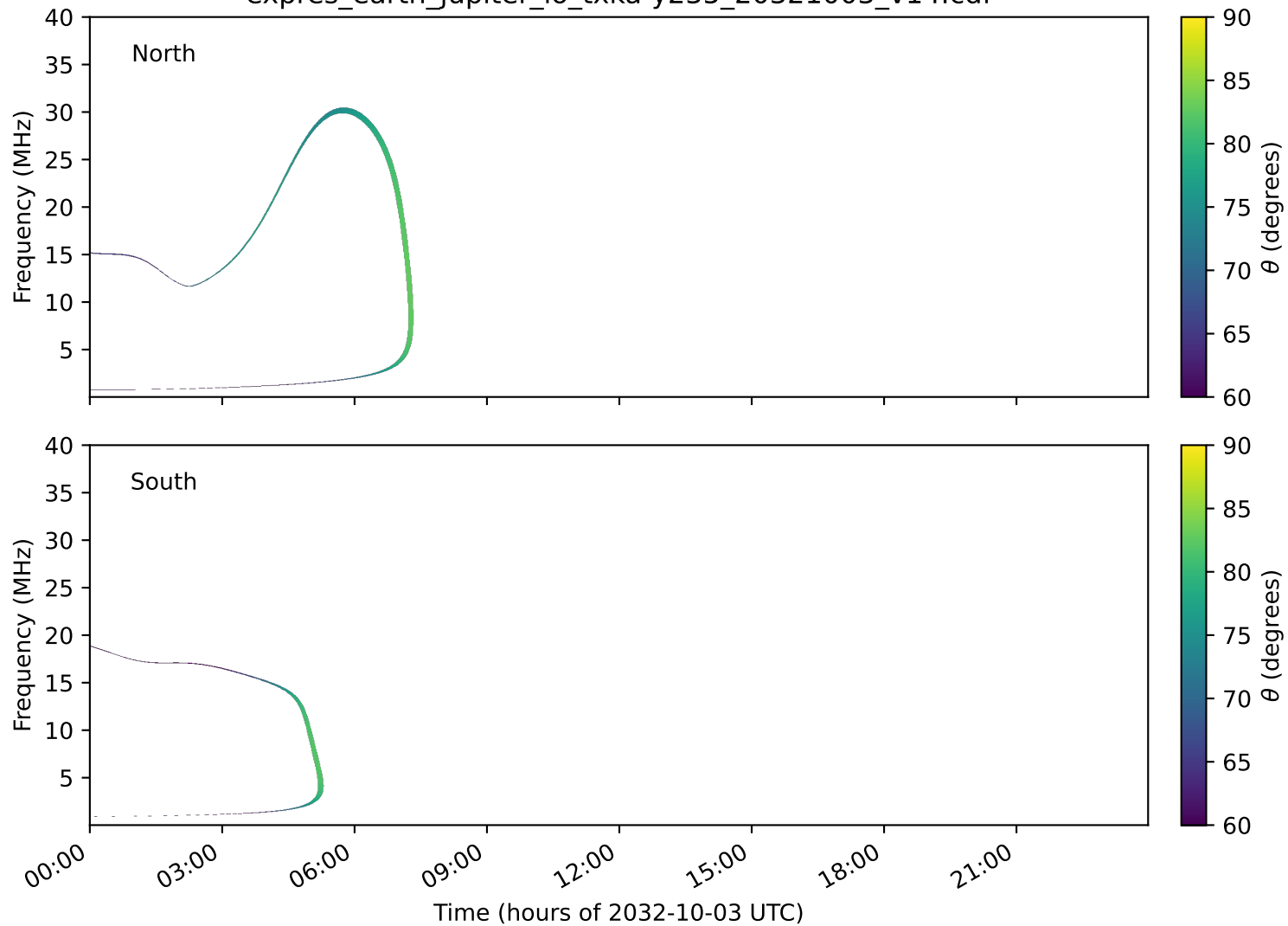
expres_earth_jupiter_io_txka-y235_20321003_v14.cdf
