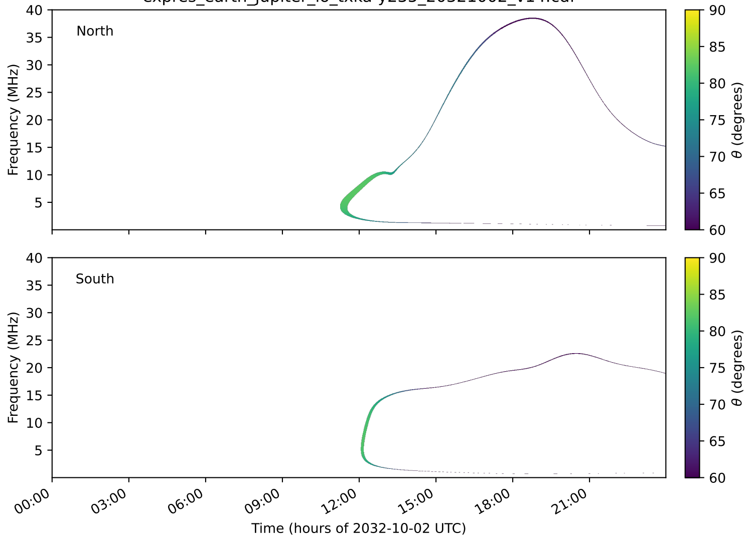
expres_earth_jupiter_io_txka-y235_20321002_v14.cdf
