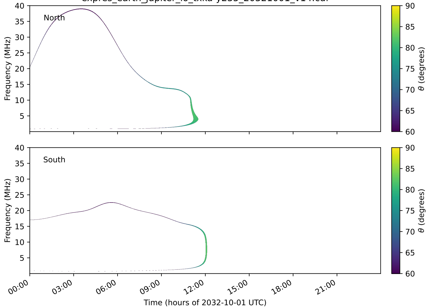
expres_earth_jupiter_io_txka-y235_20321001_v14.cdf
