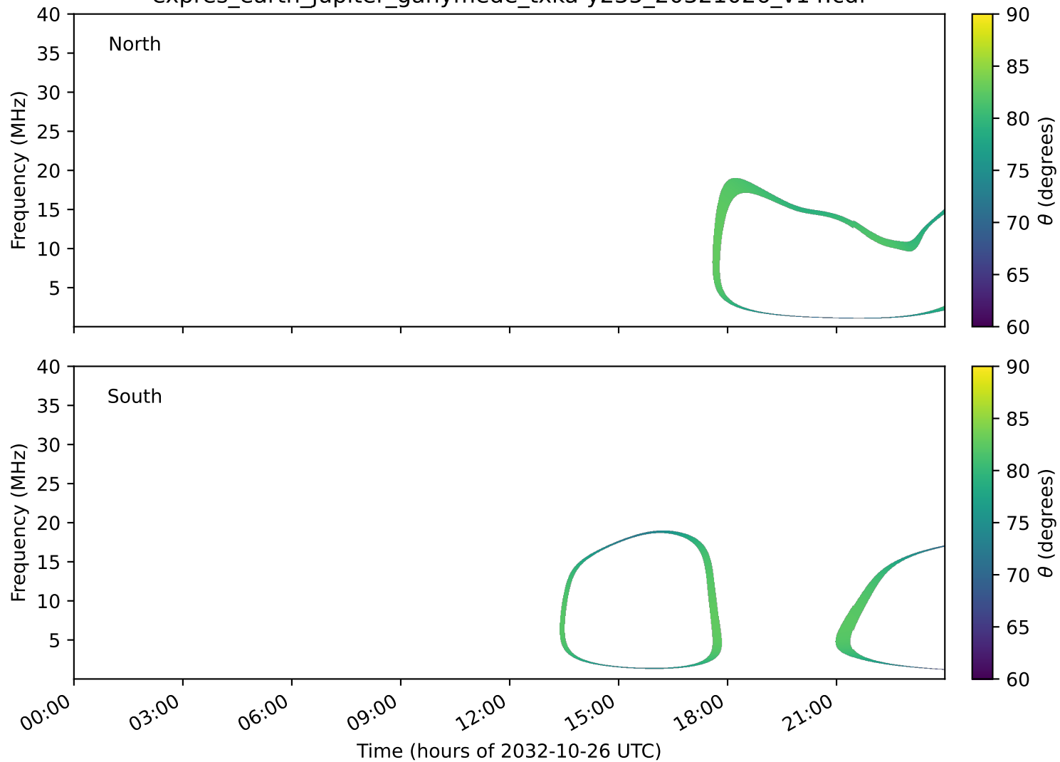
expres_earth_jupiter_ganymede_txka-y235_20321026_v14.cdf
