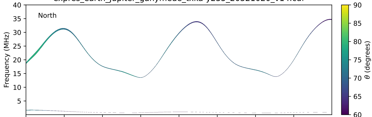
expres_earth_jupiter_ganymede_txka-y235_20321020_v14.cdf
