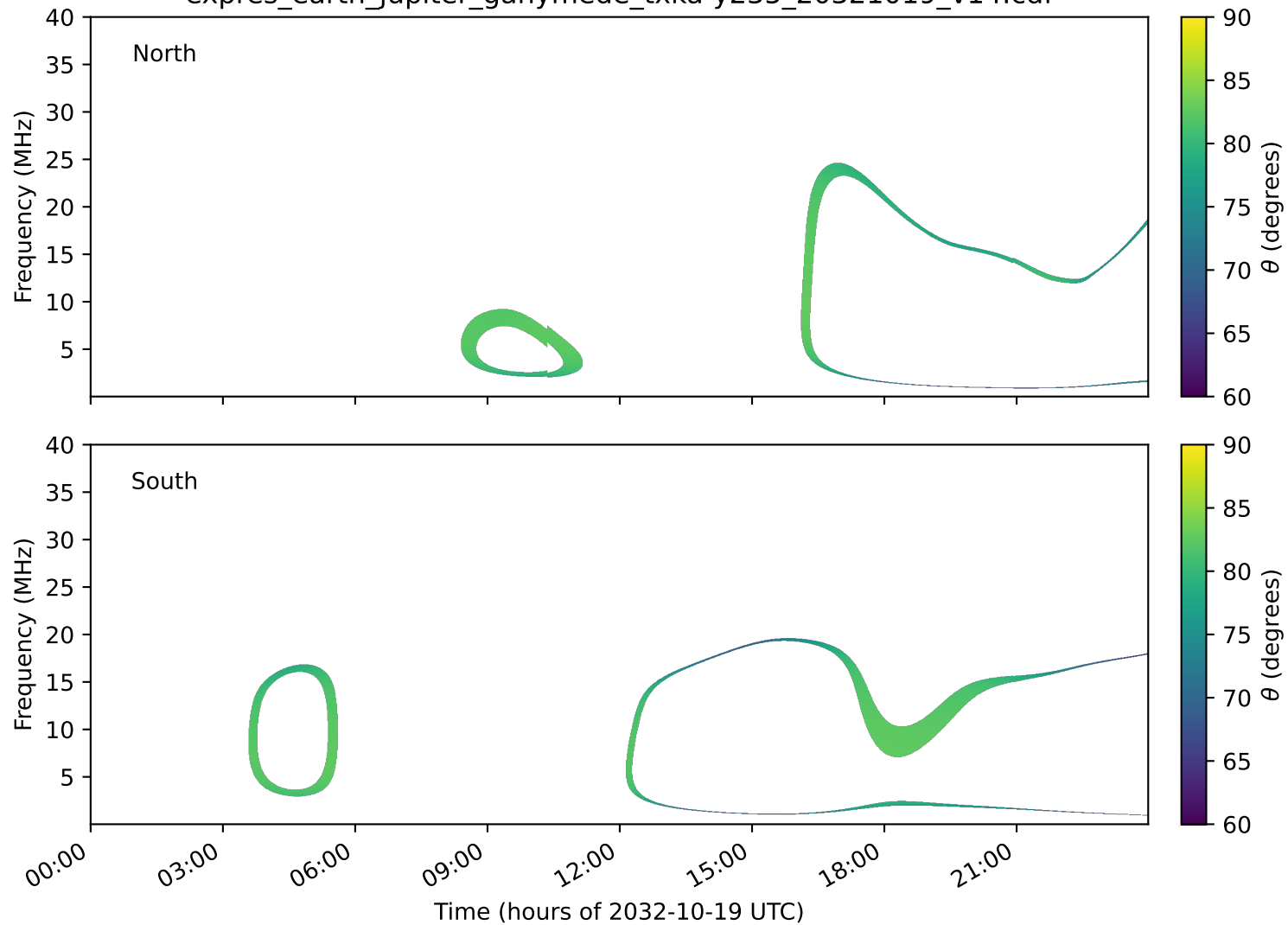
expres_earth_jupiter_ganymede_txka-y235_20321019_v14.cdf
