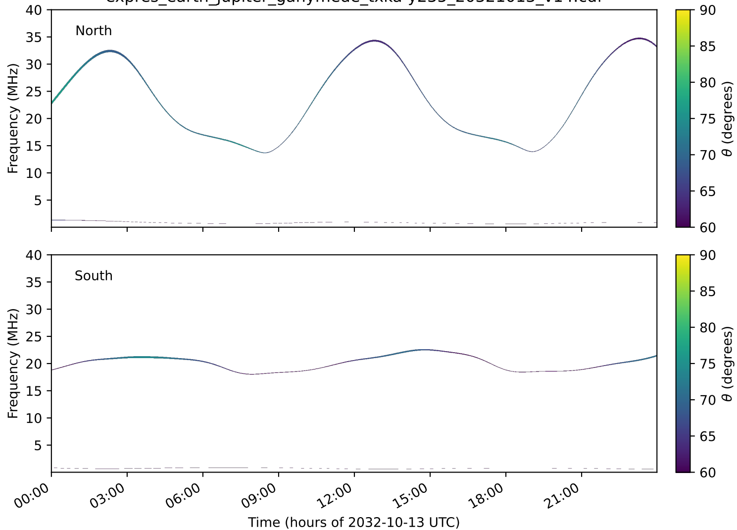
expres_earth_jupiter_ganymede_txka-y235_20321013_v14.cdf
