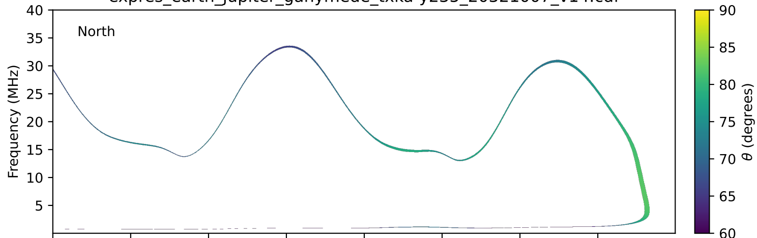
expres_earth_jupiter_ganymede_txka-y235_20321007_v14.cdf
