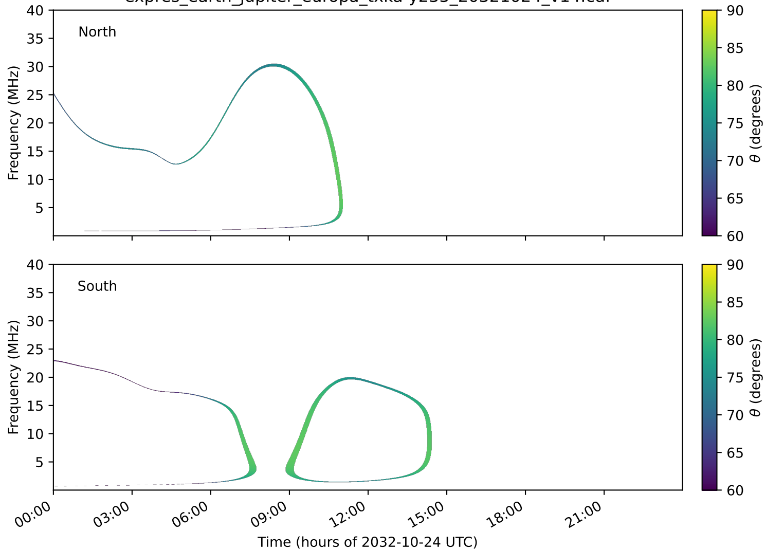
expres_earth_jupiter_europa_txka-y235_20321024_v14.cdf
