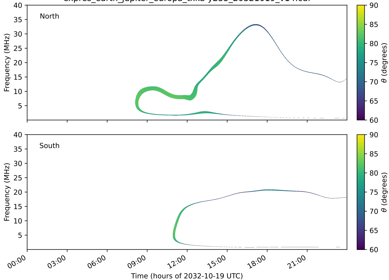
expres_earth_jupiter_europa_txka-y235_20321019_v14.cdf
