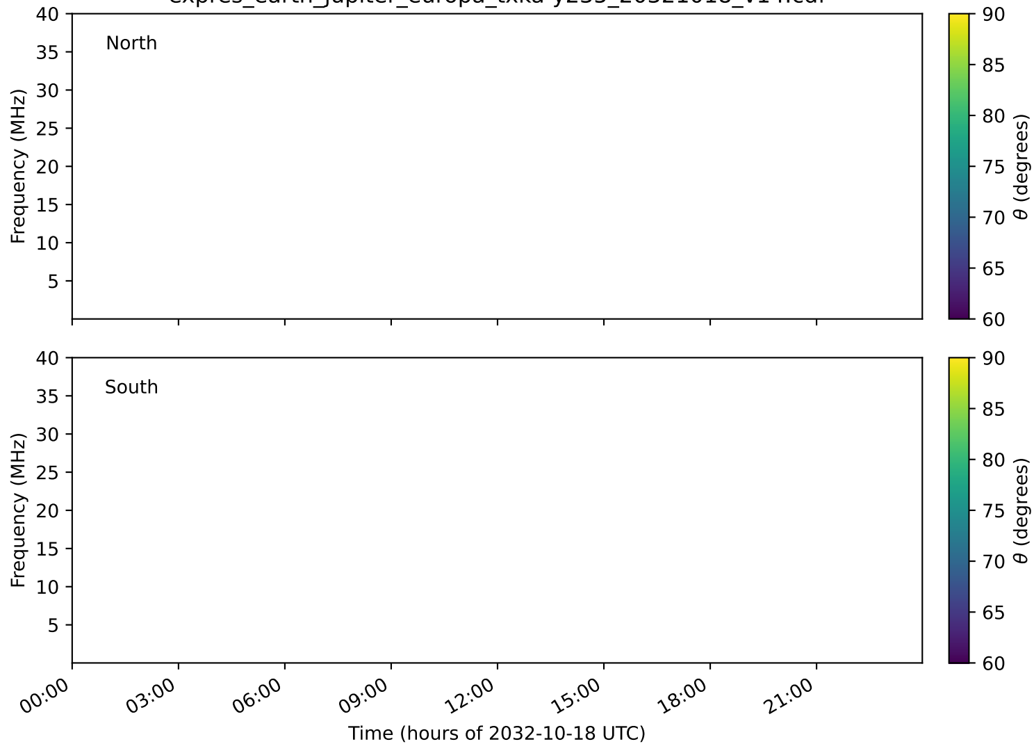
expres_earth_jupiter_europa_txka-y235_20321018_v14.cdf
