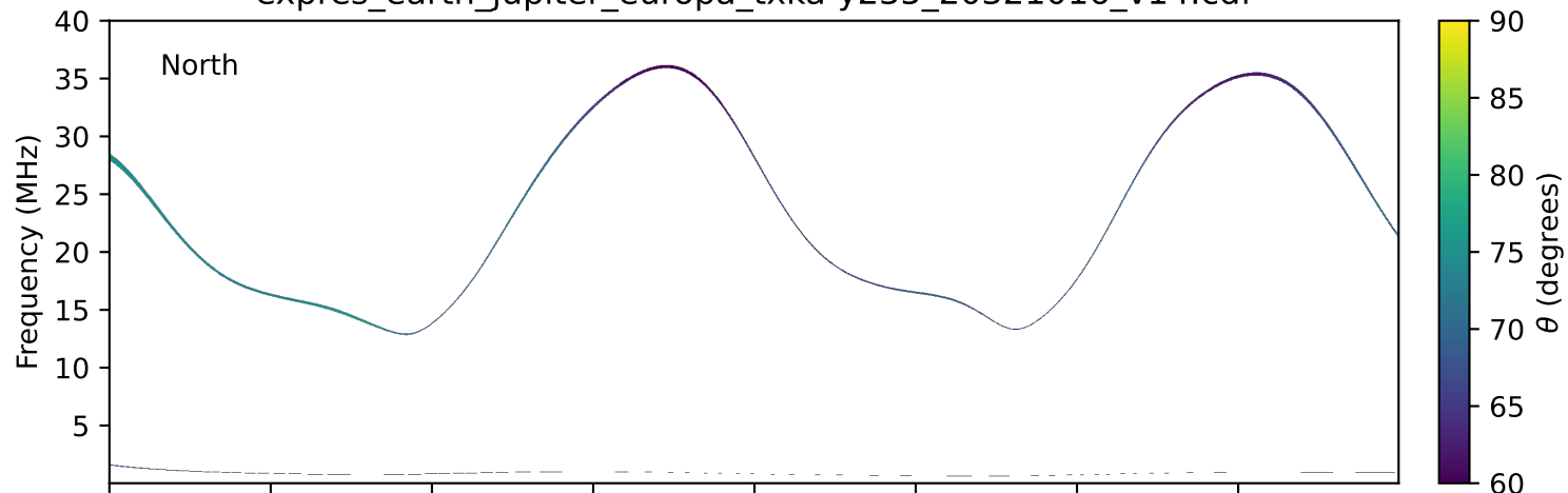
expres_earth_jupiter_europa_txka-y235_20321016_v14.cdf
