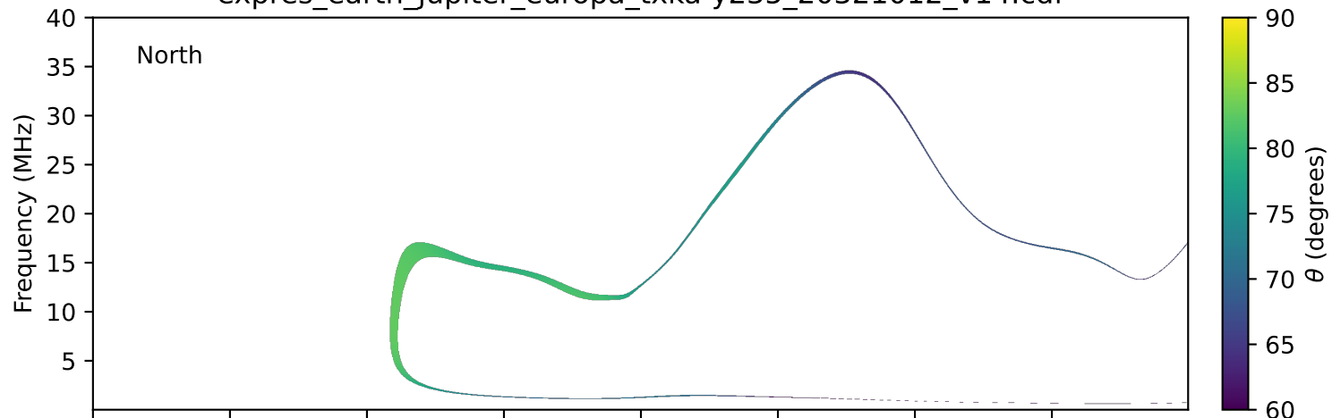
expres_earth_jupiter_europa_txka-y235_20321012_v14.cdf
