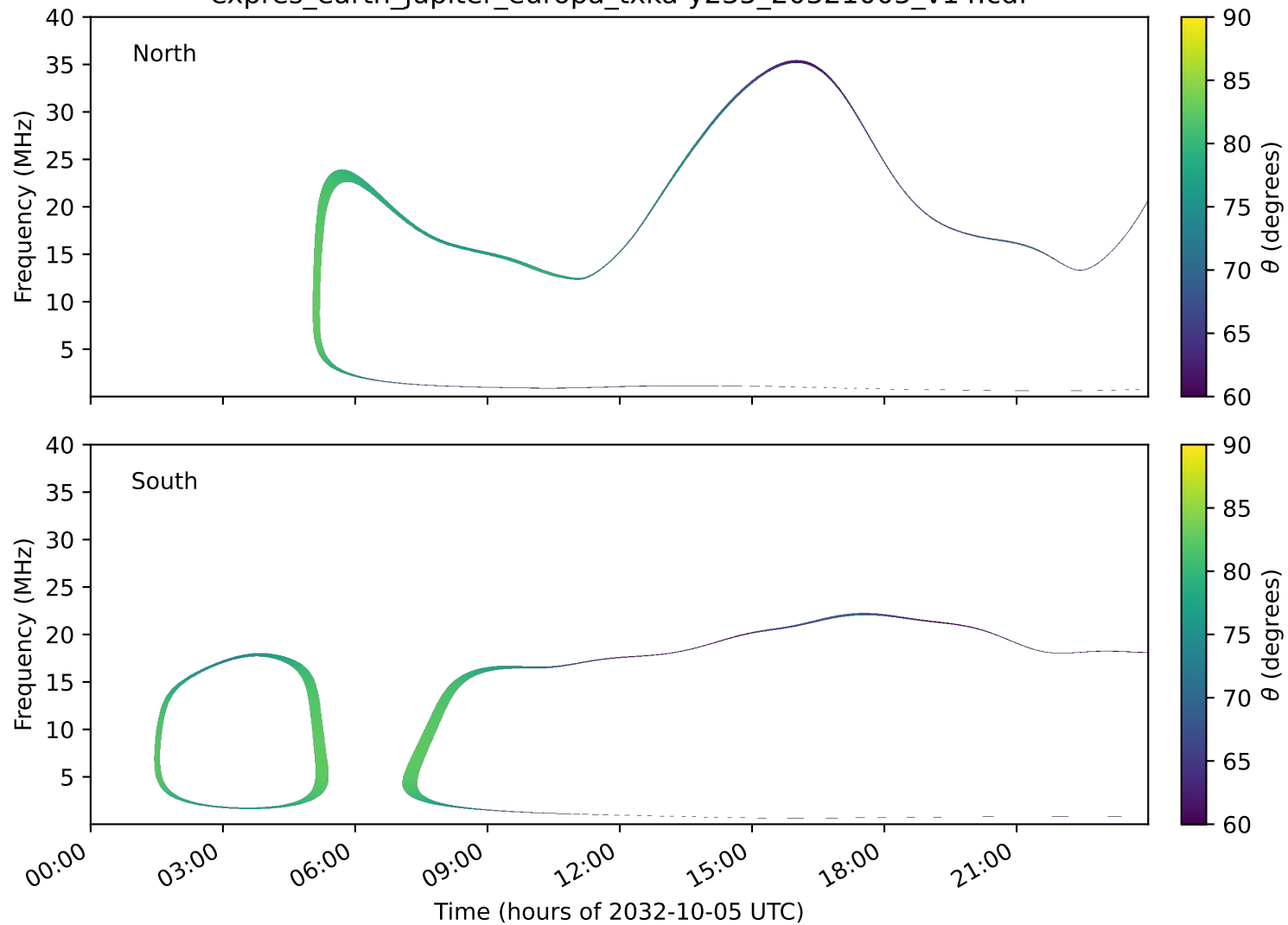
expres_earth_jupiter_europa_txka-y235_20321005_v14.cdf
