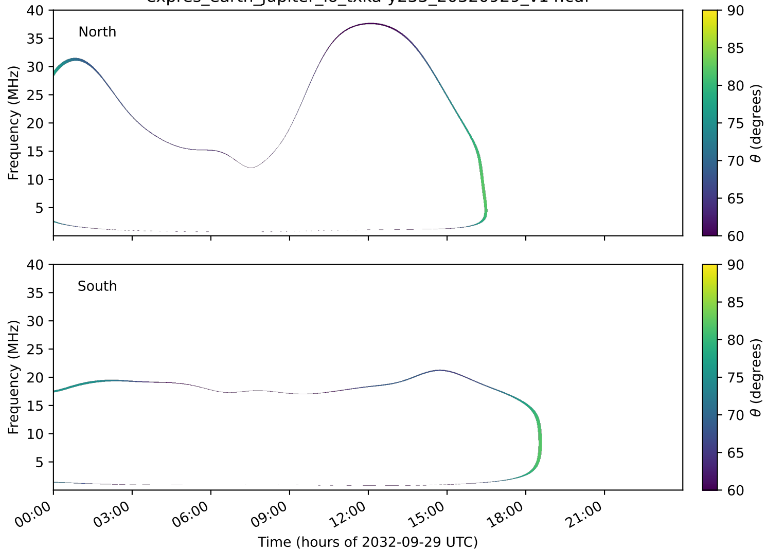
expres_earth_jupiter_io_txka-y235_20320929_v14.cdf
