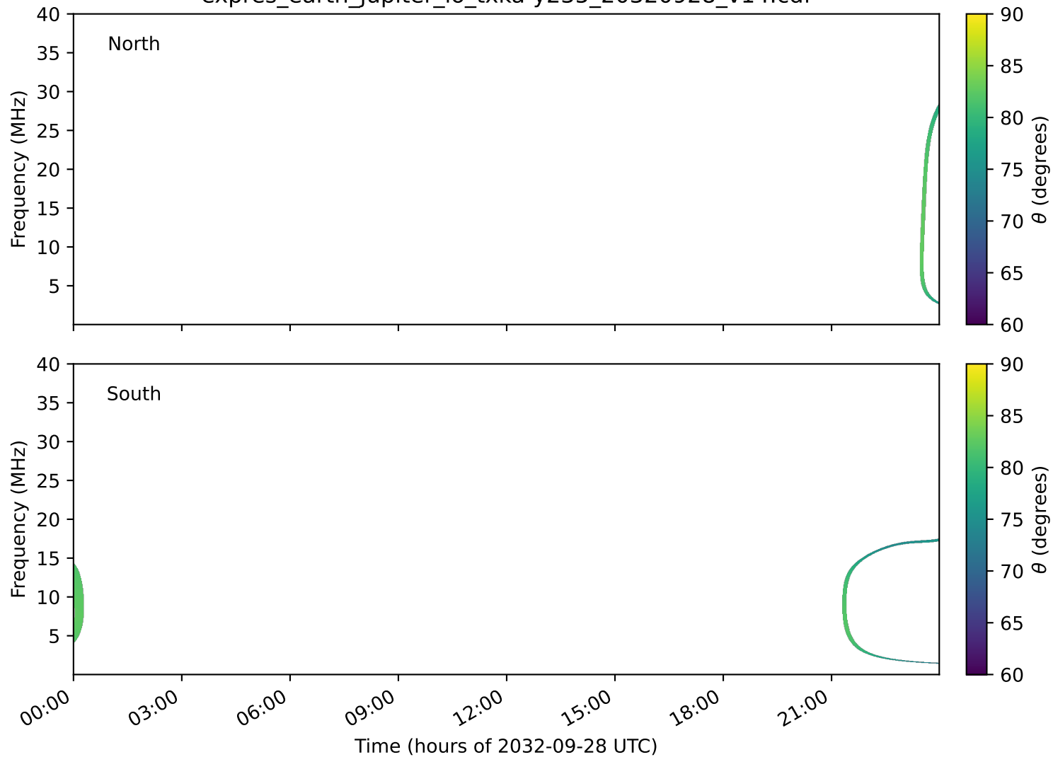
expres_earth_jupiter_io_txka-y235_20320928_v14.cdf
