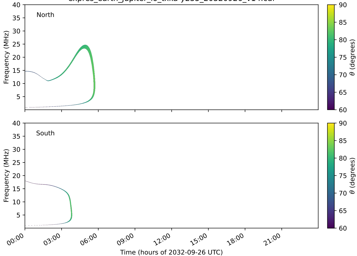
expres_earth_jupiter_io_txka-y235_20320926_v14.cdf
