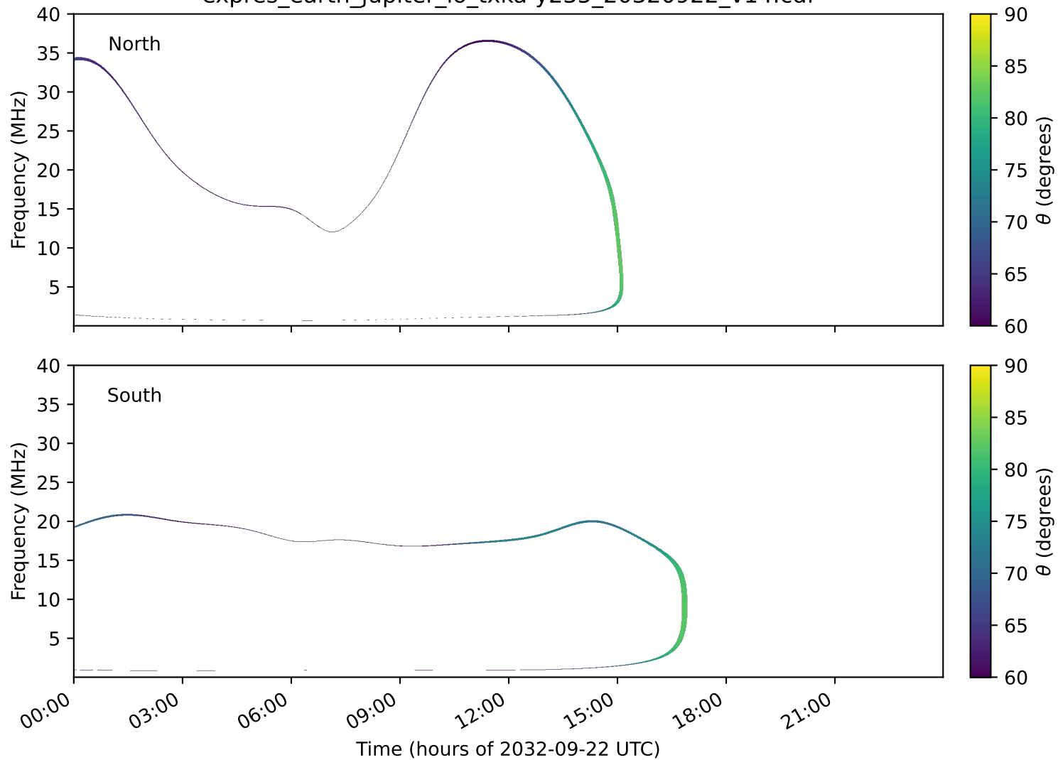
expres_earth_jupiter_io_txka-y235_20320922_v14.cdf
