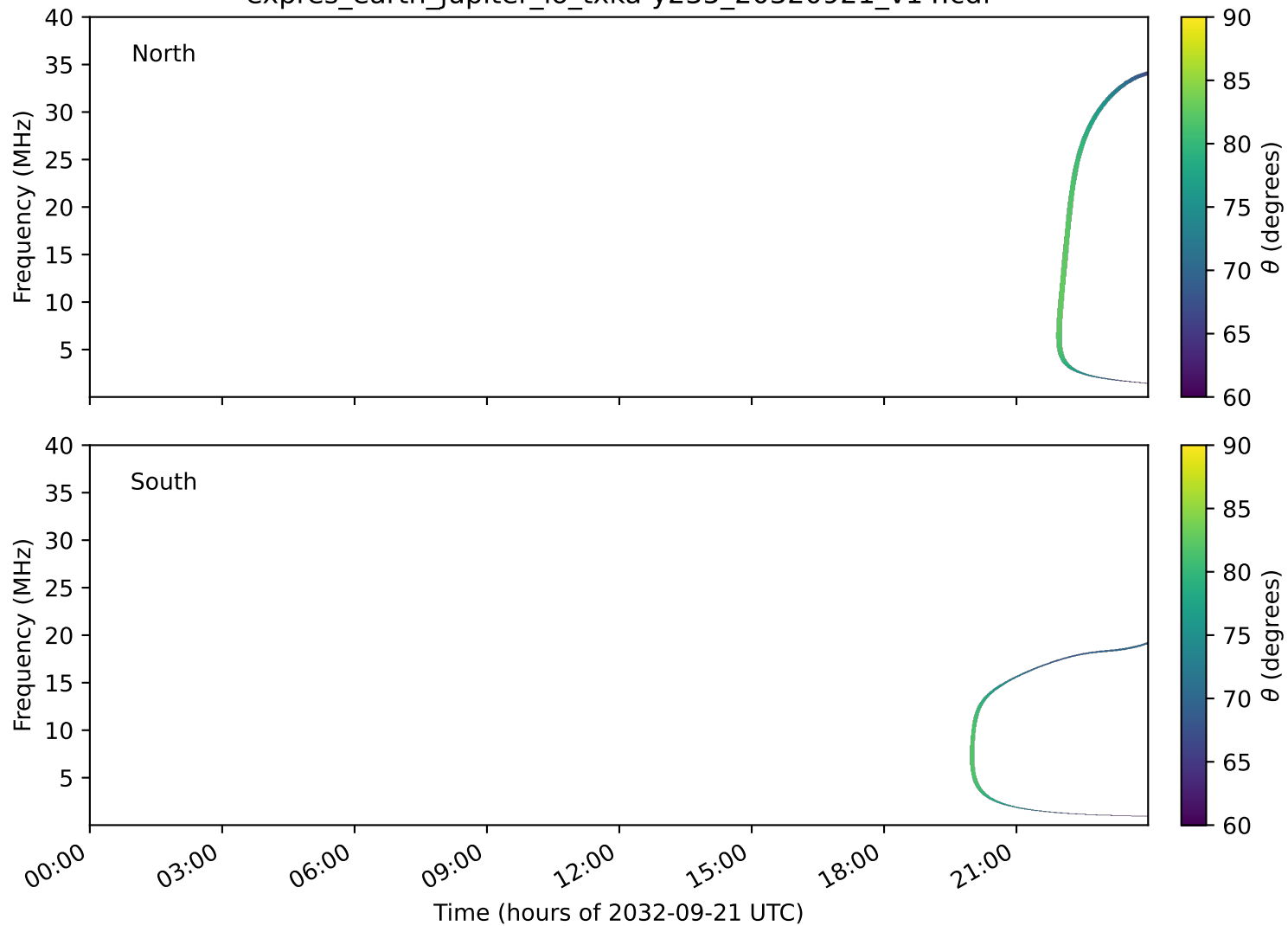
expres_earth_jupiter_io_txka-y235_20320921_v14.cdf
