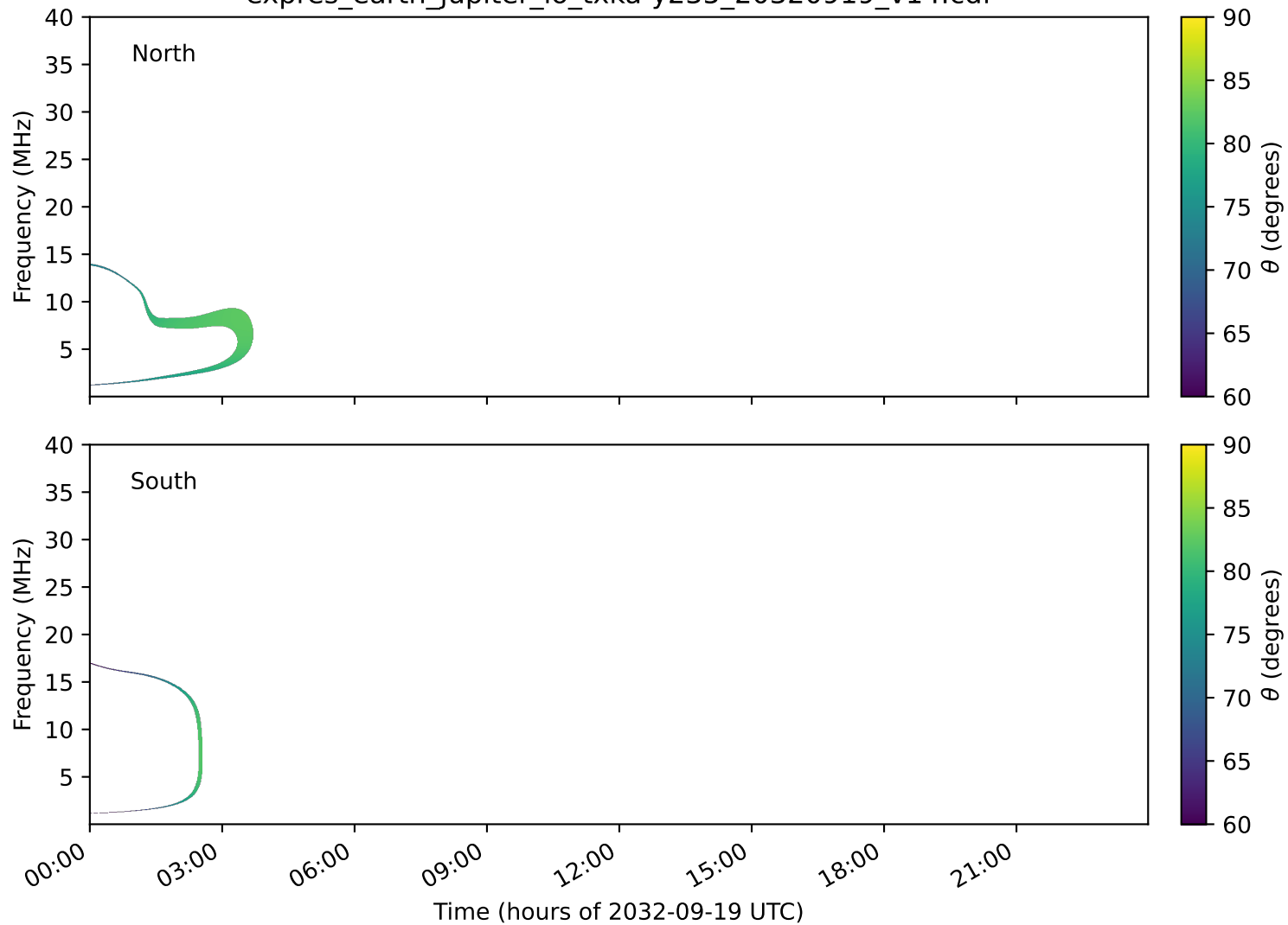
expres_earth_jupiter_io_txka-y235_20320919_v14.cdf
