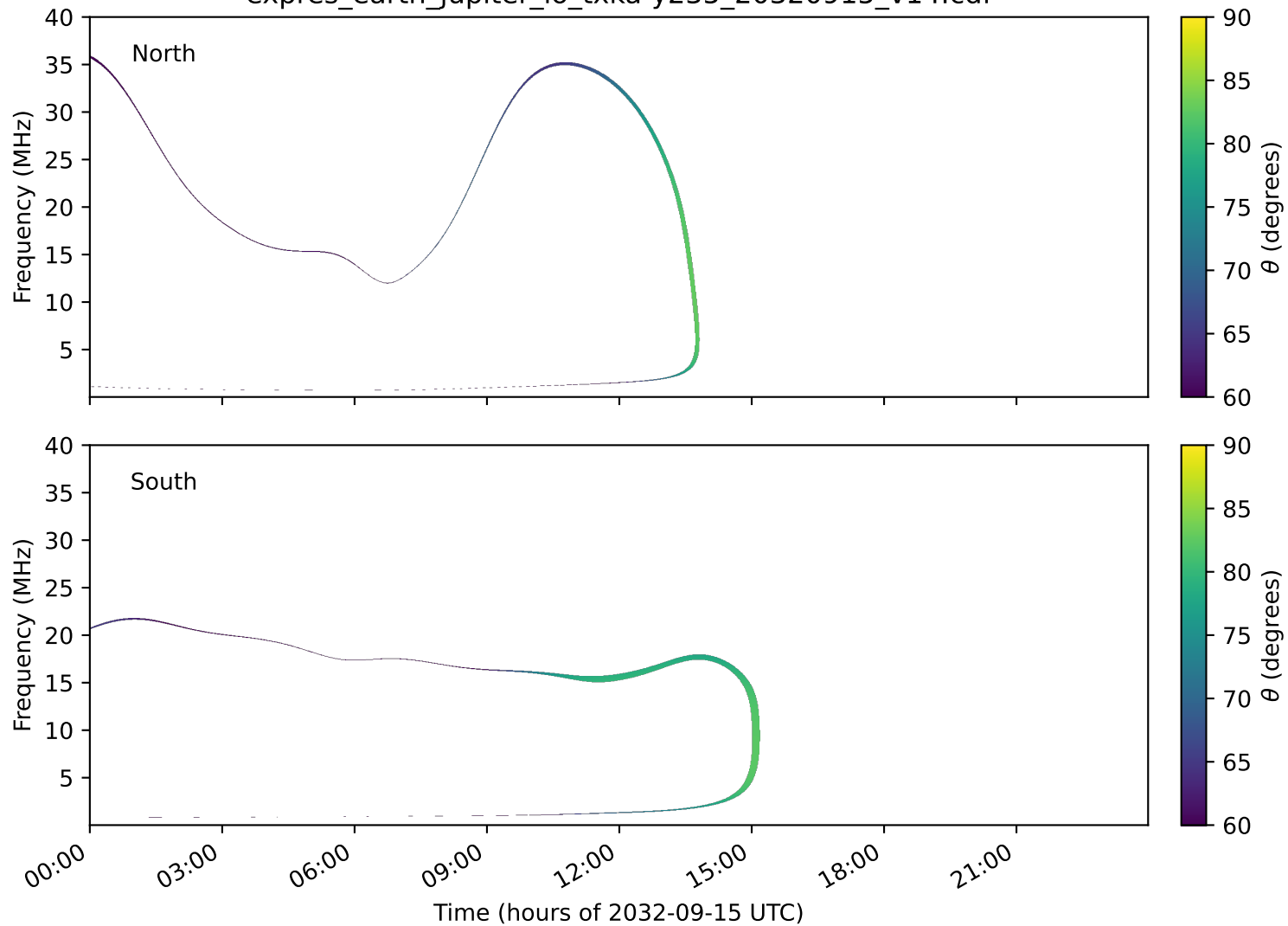
expres_earth_jupiter_io_txka-y235_20320915_v14.cdf
