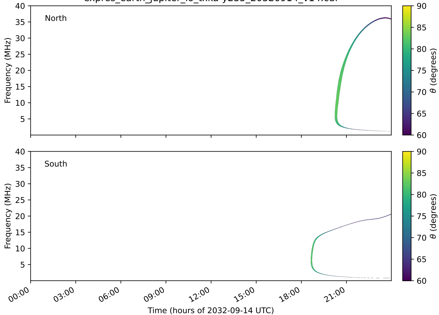
expres_earth_jupiter_io_txka-y235_20320914_v14.cdf
