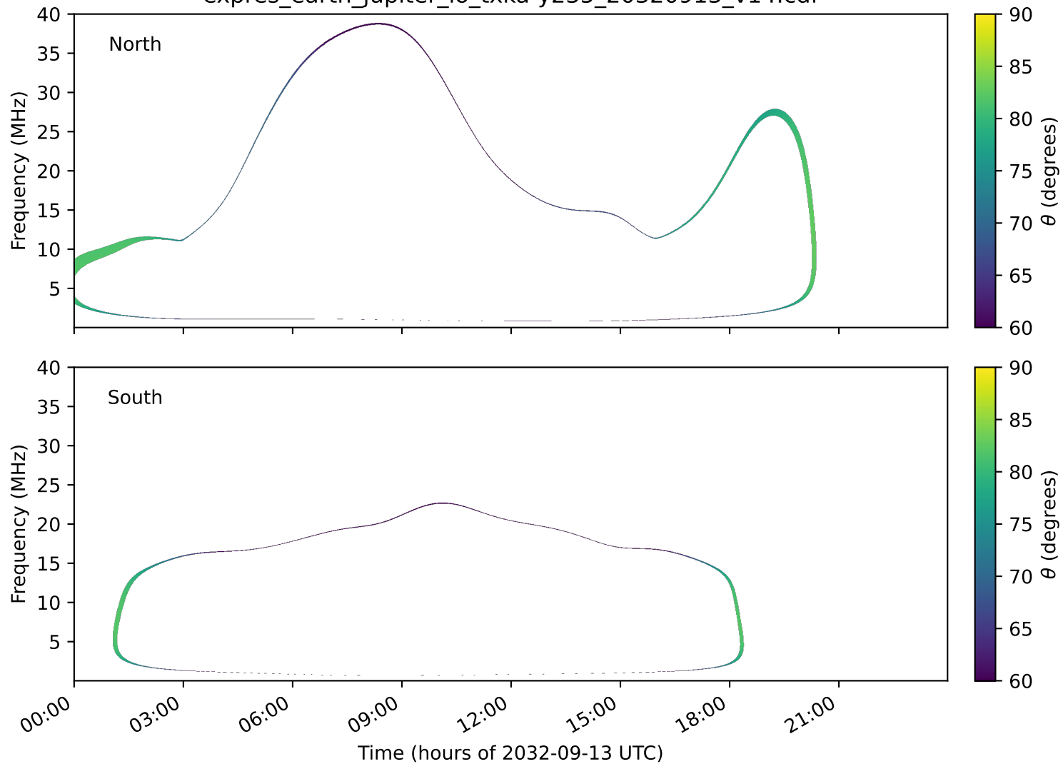
expres_earth_jupiter_io_txka-y235_20320913_v14.cdf
