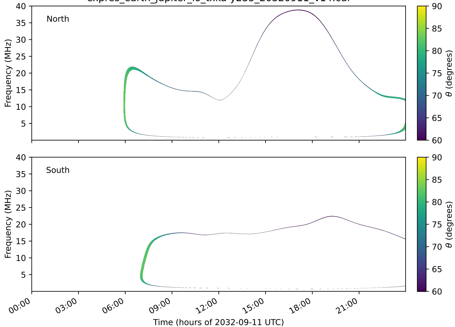
expres_earth_jupiter_io_txka-y235_20320911_v14.cdf
