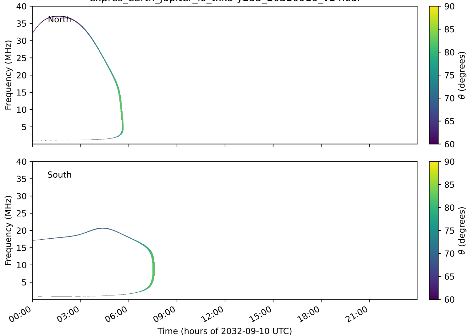
expres_earth_jupiter_io_txka-y235_20320910_v14.cdf
