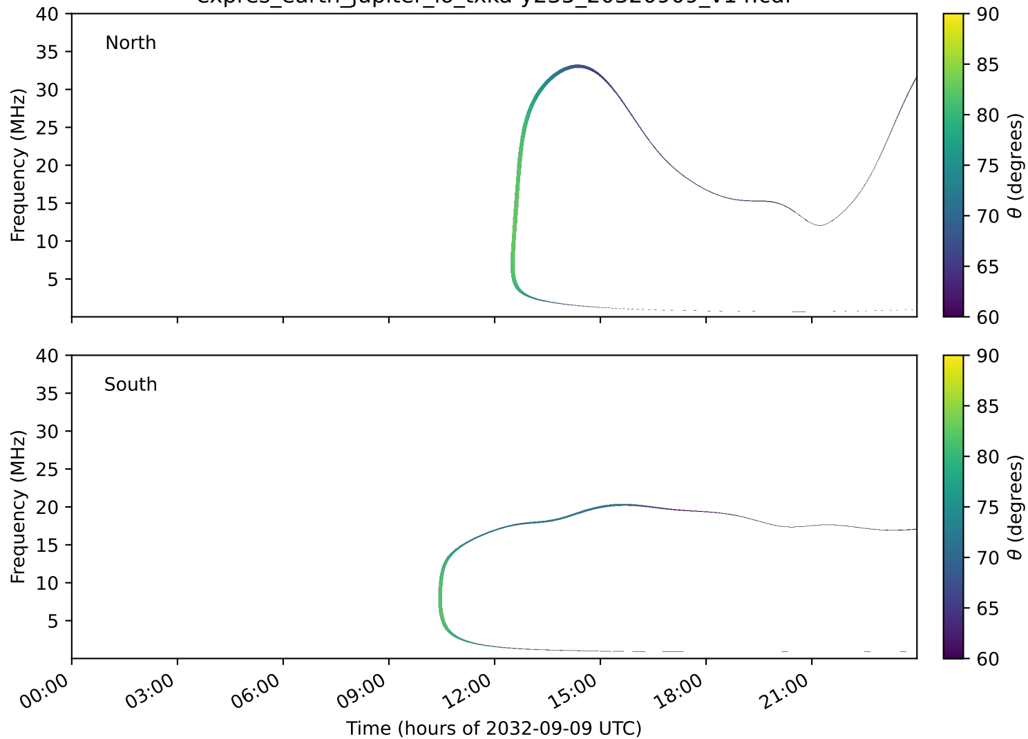
expres_earth_jupiter_io_txka-y235_20320909_v14.cdf
