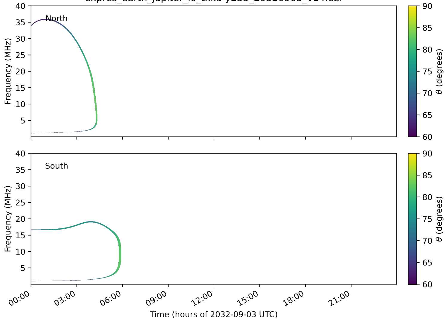
expres_earth_jupiter_io_txka-y235_20320903_v14.cdf
