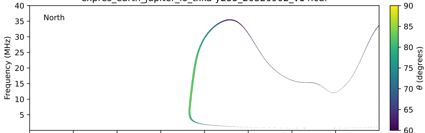
expres_earth_jupiter_io_txka-y235_20320902_v14.cdf
