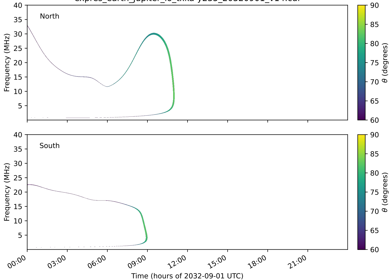
expres_earth_jupiter_io_txka-y235_20320901_v14.cdf
