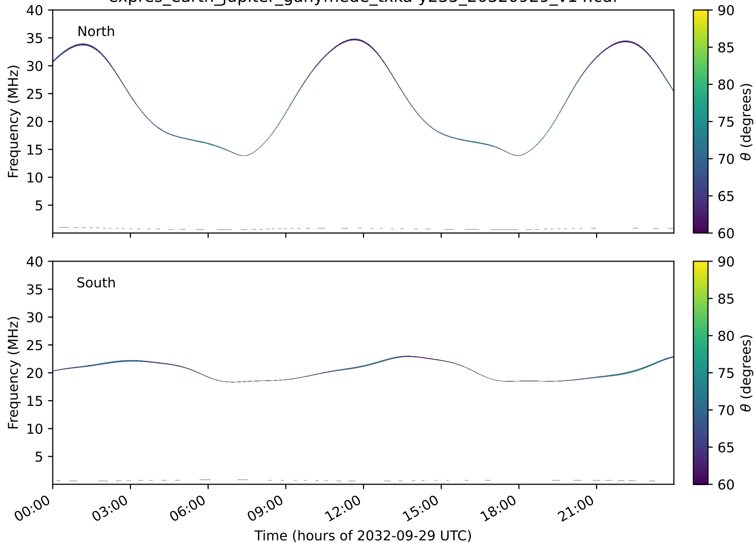
expres_earth_jupiter_ganymede_txka-y235_20320929_v14.cdf
