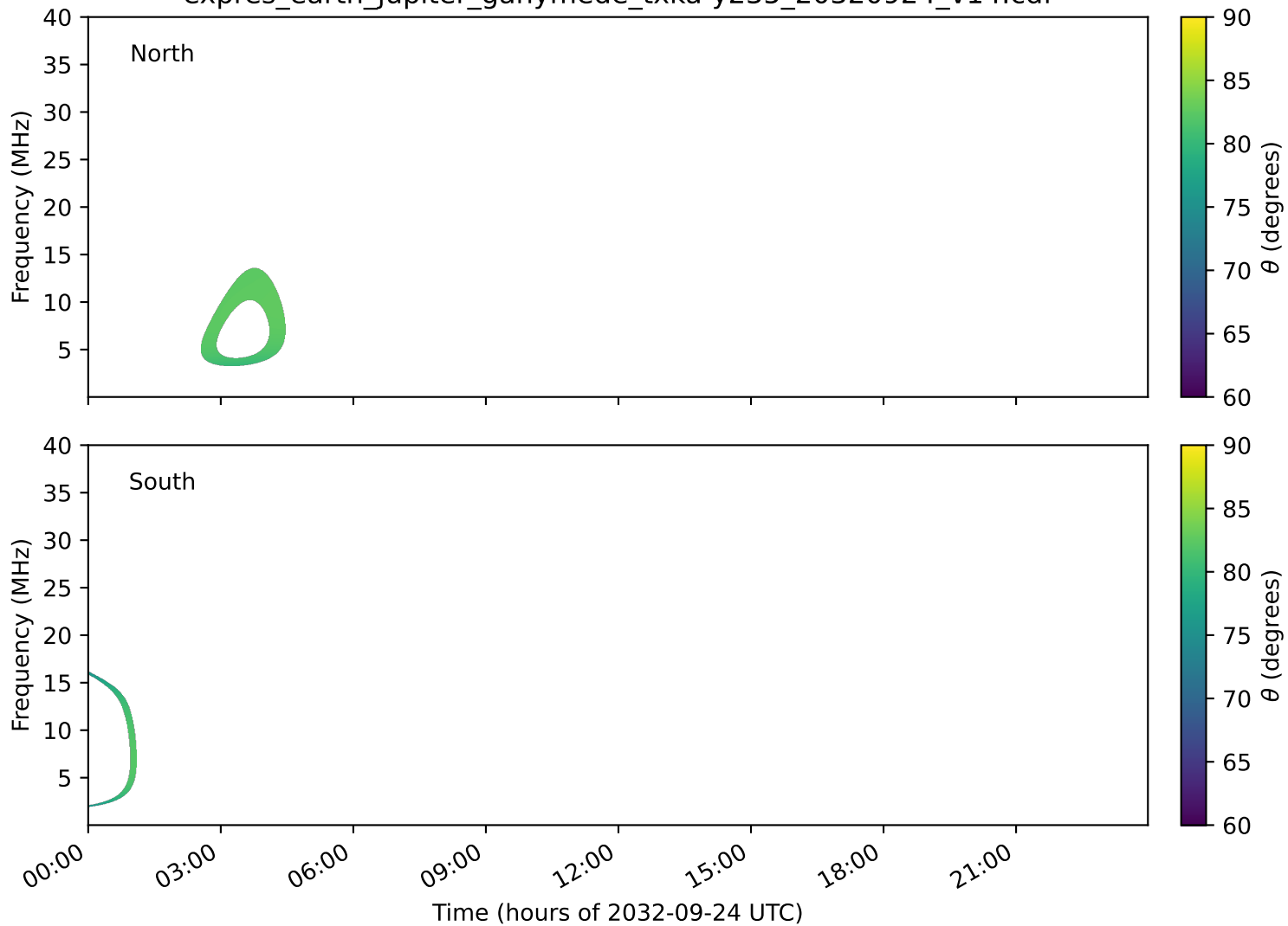
expres_earth_jupiter_ganymede_txka-y235_20320924_v14.cdf
