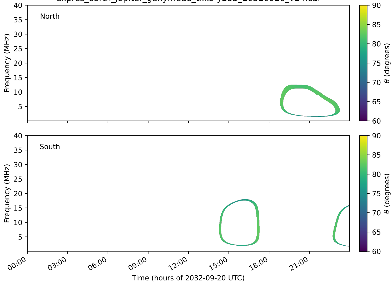
expres_earth_jupiter_ganymede_txka-y235_20320920_v14.cdf
