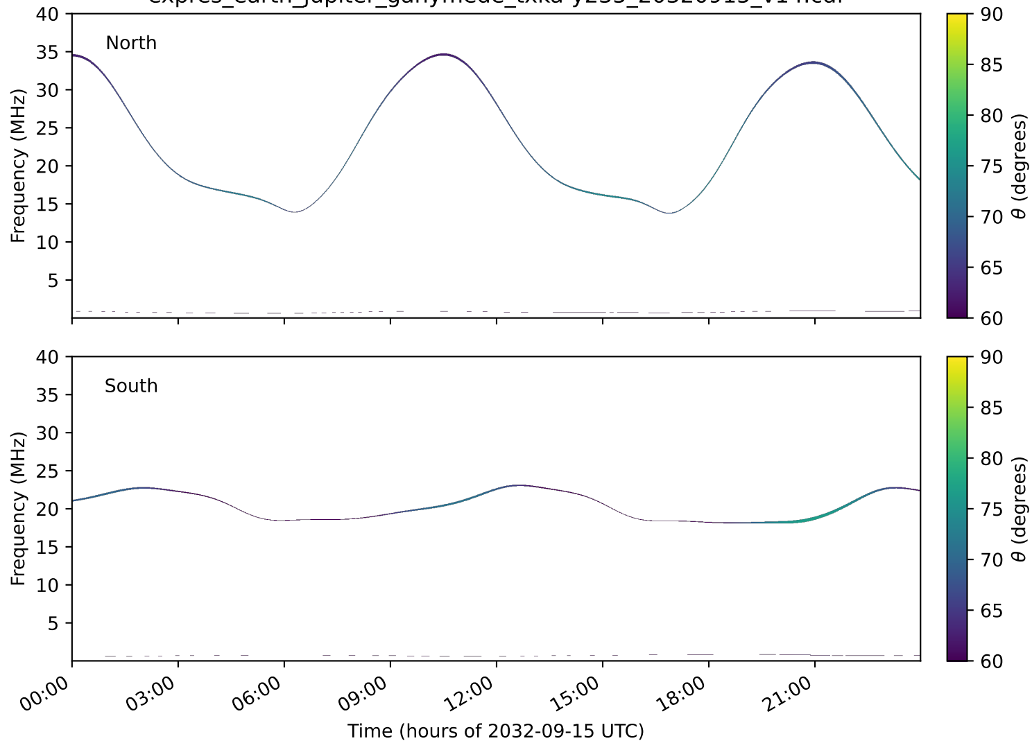
expres_earth_jupiter_ganymede_txka-y235_20320915_v14.cdf
